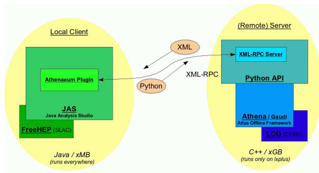
Figure 1: Athenaeum Architecture.
